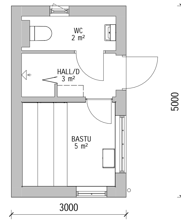
PLAN
